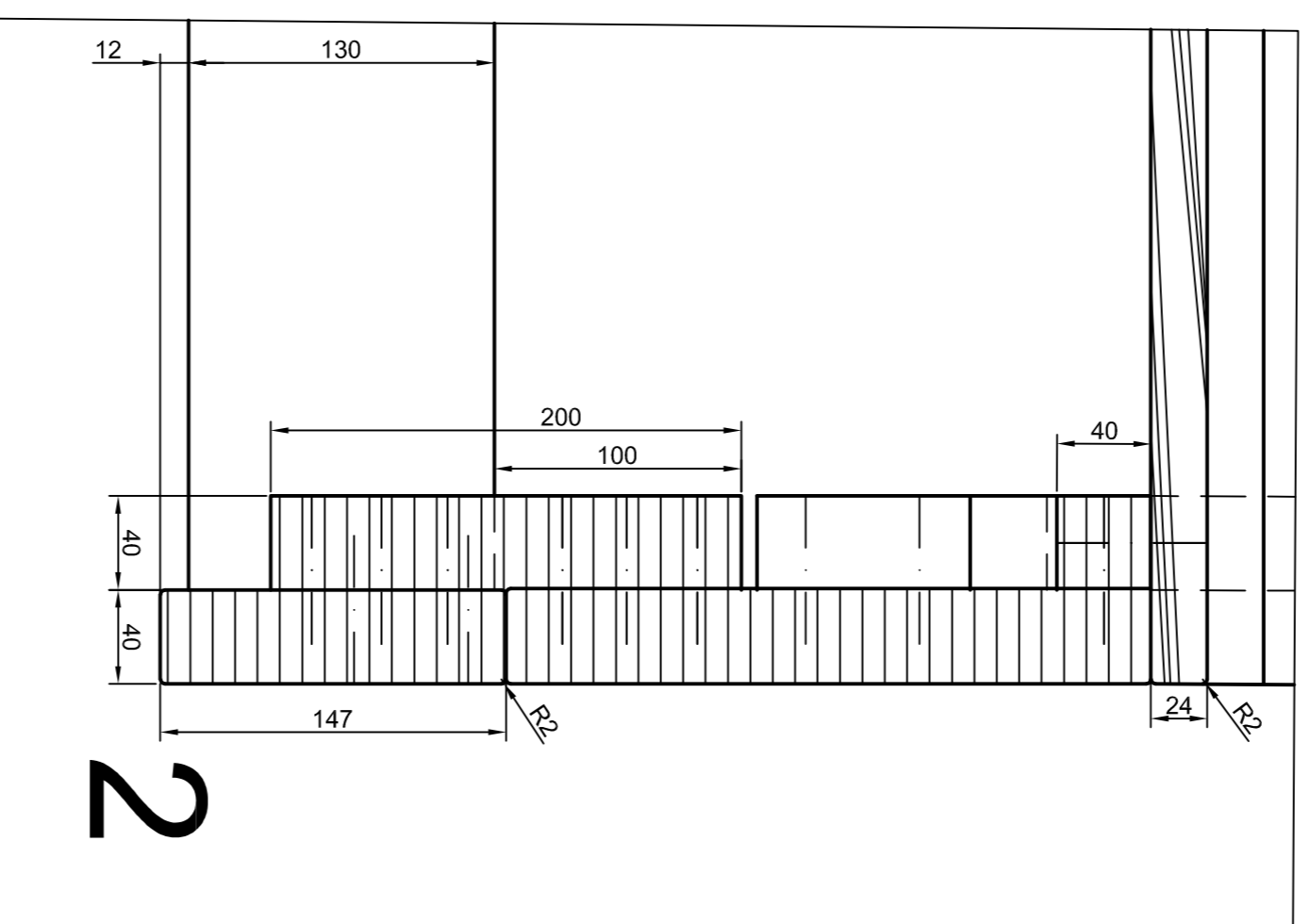
2. junction M 1:3
