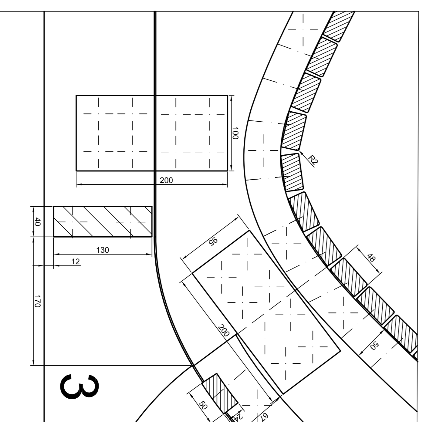
3. junction M 1:3
